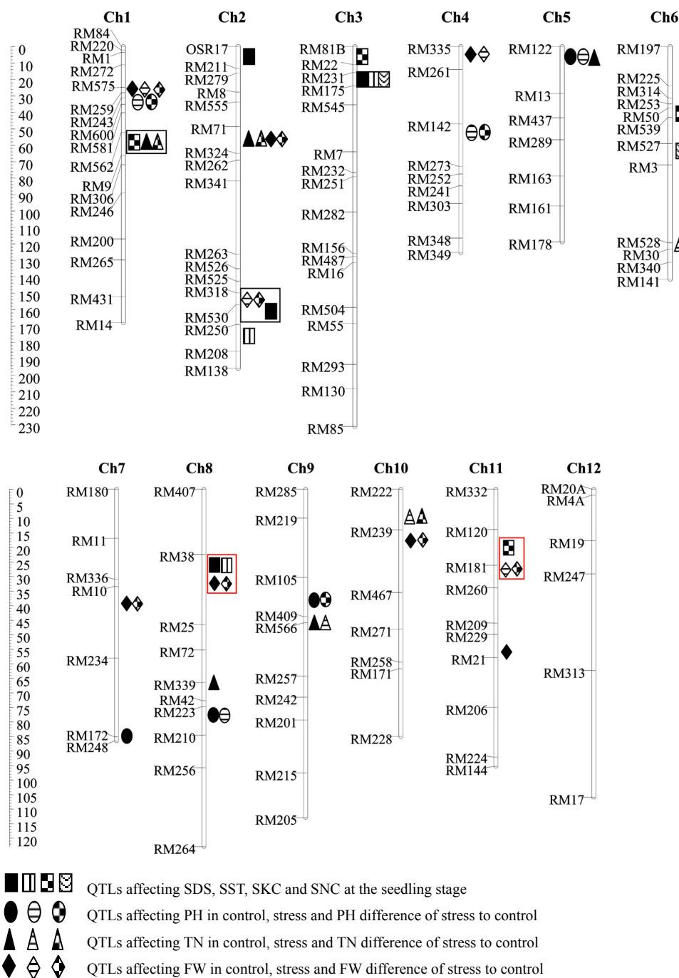
Figure 1 QTLs affecting survival days of seedlings (SDS), score of salt toxicity of leaves (SST), shoot K^+ concentration (SKC) and shoot Na^+ concentration (SNC) at the seedling stage, and plant height (PH), tiller number (TN) and fresh weight of shoots (FW) at the tillering stage detected in IR64/Binam BC_2F_8 introgression lines. QTLs in rectangles mean genetic overlapping QTLs underlying ST of seedling and tillering stages.
