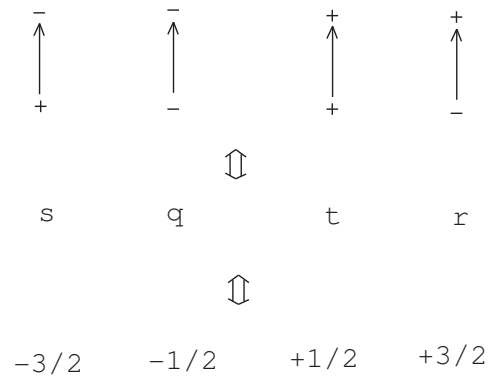
FIG. 5: the bottom row represents the spin eigenvalues
