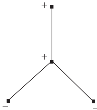
FIG. 3: An up-spin which has only a single up-spin neighbor. This is energetically penalized by K = \sum_p K_p .
