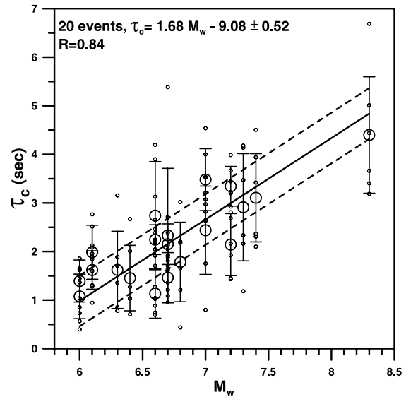
Fig. 1. \tau_c estimates for 20 events using the nearest 6 stations of K-NET and KiK-net. Small open circles show single-record results and large circles show the event-average. Solid line shows the least squares fit and the two dashed lines show the range of one standard deviation.
