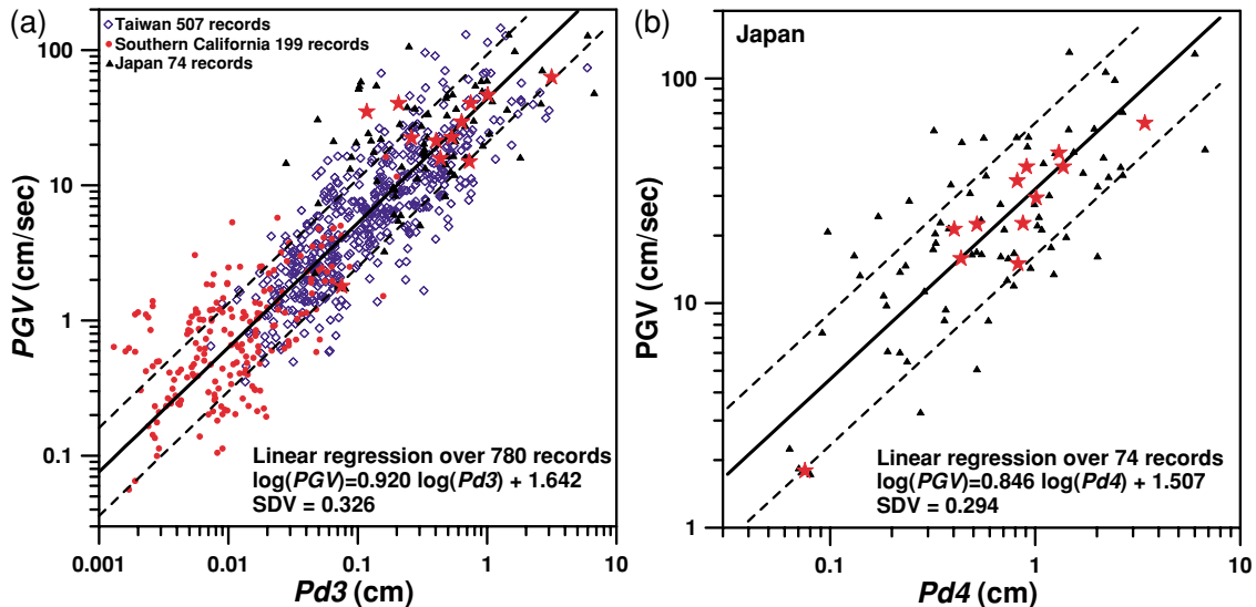
Fig. 2. (a) Relationship between peak initial three-second displacement amplitude ( Pd3 ) and peak ground velocity (PGV) for 780 records with the epicentral distances less than 30 km for Japan (black triangles), southern California (red solid circles) and Taiwan (blue diamonds). Red stars indicate the event-average of the Japanese data. Solid line indicates the least squares fit and the two dashed lines show the range of one standard deviation. (b) Relationship between peak initial four-second displacement amplitude ( Pd4 ) and PGV. Red stars indicate the event-average of the Japanese data. Solid line indicates the least squares fit and the two dashed lines show the range of one standard deviation.
