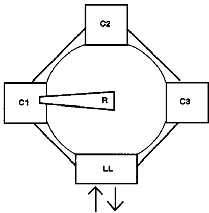
Fig. 2. An outline of a 3-chamber cluster tool.
