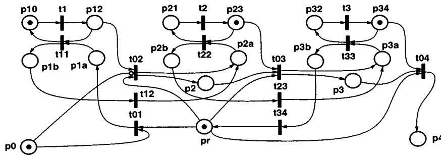
Fig. 10. Petri net model for final transient behavior of a dual-blade 3-chamber tool.
