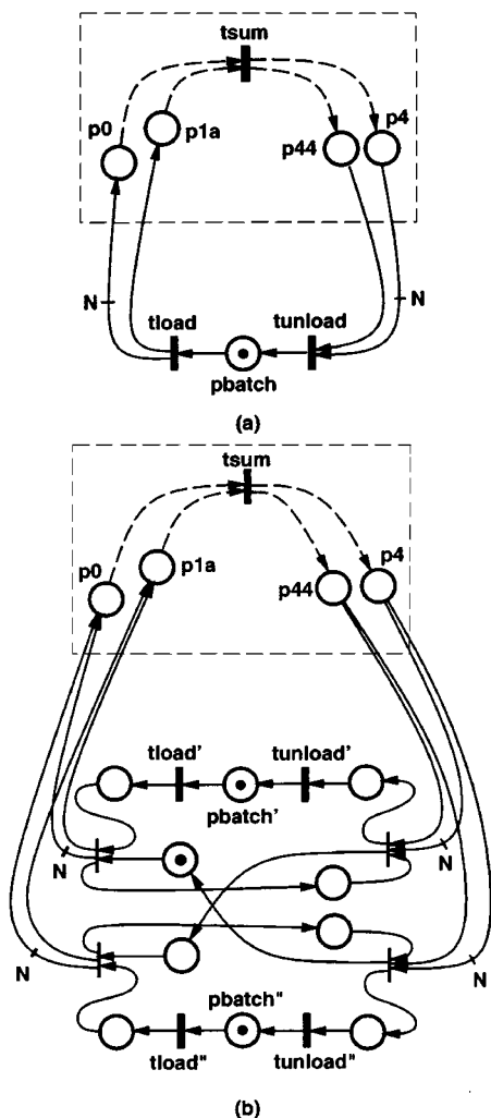
Fig. 12. Outline of a model for a cluster tool with (a) single loadlock and (b) with two loadlocks.
