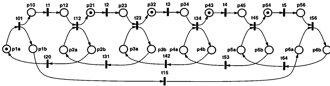
Fig. 17. Petri net model for the steady-state behavior of a single-blade 5-chamber cluster tool.
