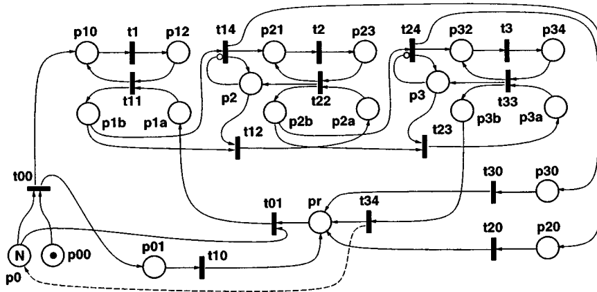
Fig. 9. Petri net model for initial transient behavior of a dual-blade 3-chamber tool.
