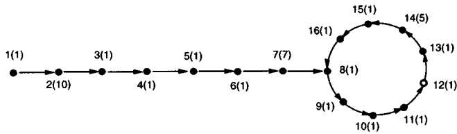
Fig. 5. State graph for the modified net of Fig. 4.
