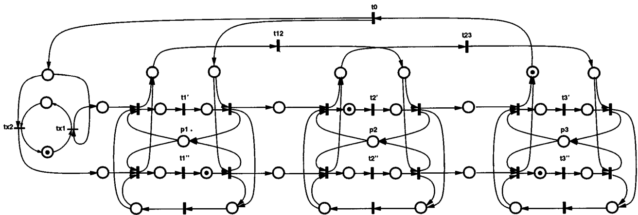
Fig. 20. Petri net model for a dual-blade 3-chamber cluster tool with two types of wafers.
