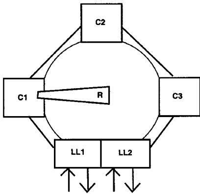
Fig. 11. An outline of a 3-chamber 2-loadlock cluster tool.
