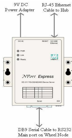
Fig. 6. DE-311 Serial Server (Image Courtesy: Moxa Technologies).
