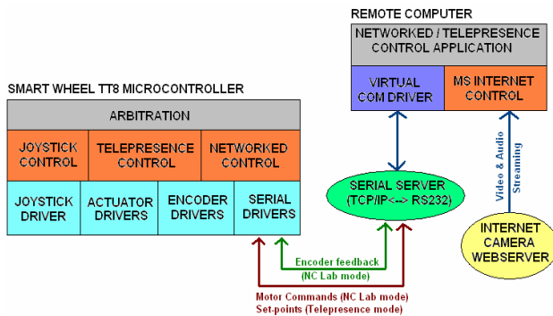
Fig. 8. Smart Wheel Software Architecture.
