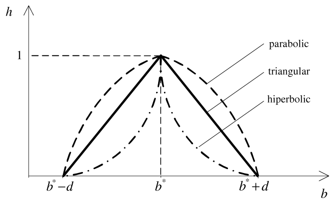
Fig. 2. The examples of the certainty distributions
